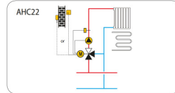
Mixing heating circuit, room temperature or/and weather compensated control.
