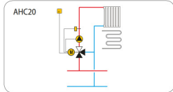
Mixing heating circuit, room temperature control.
