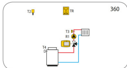
Mixing heating circuit, weather compensated control.
